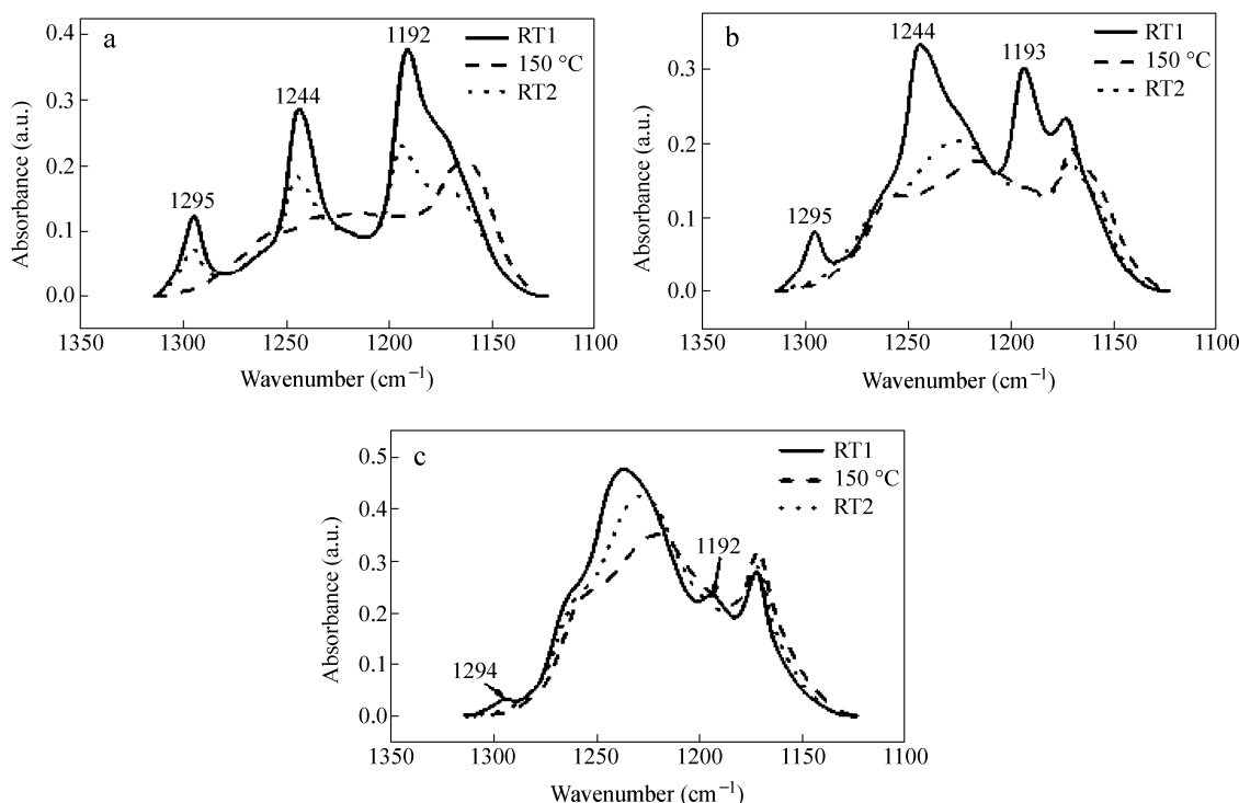
Fig. 3 FTIR spectra in the region from 1314 \text{cm}^{-1} to 1123 \text{cm}^{-1} of PCL/PVPh films of different blend compositions: (a) 80/20, (b) 50/50 and (c) 20/80. The samples were first cast from THF and recorded at room temperature (solid line), then heated at 150 ^{\circ}\text{C} for 5 min (dashed line) and cooled to RT again (dotted line).
